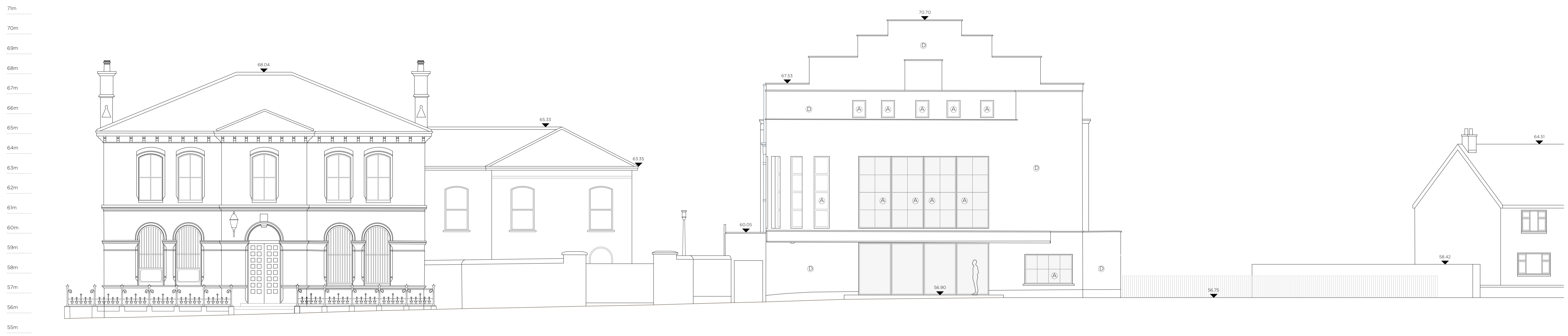
NORTH ELEVATION _ PROPOSED
