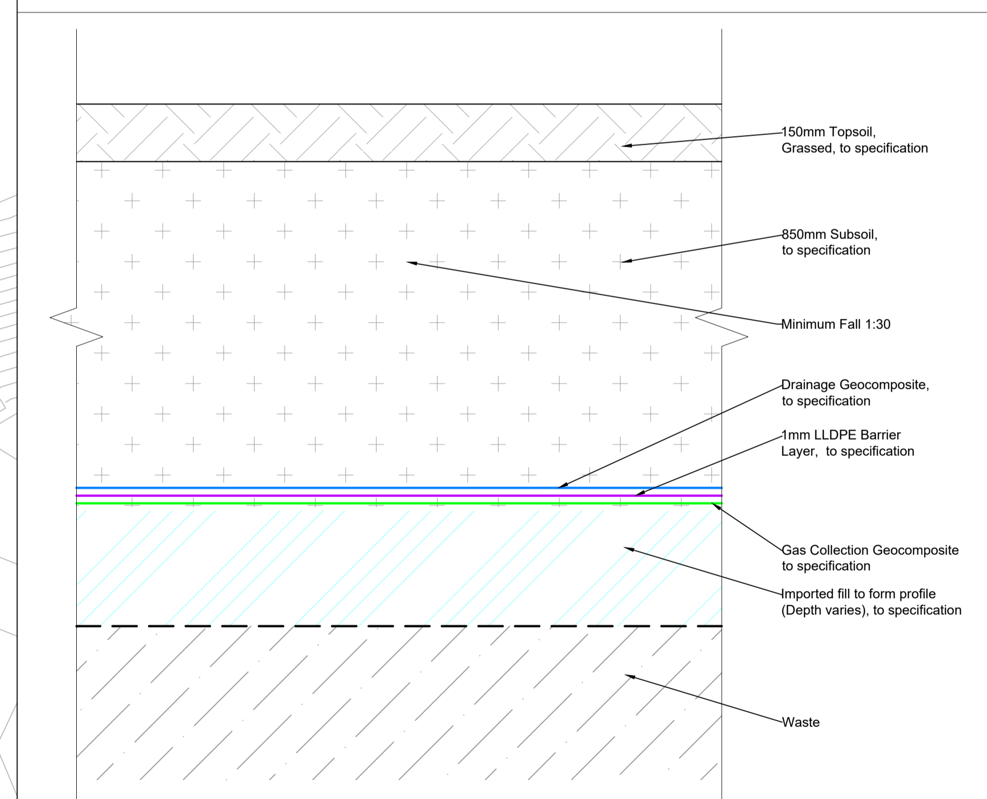
TYPICAL CAPPING DETAIL - WITHOUT GEOGRID
