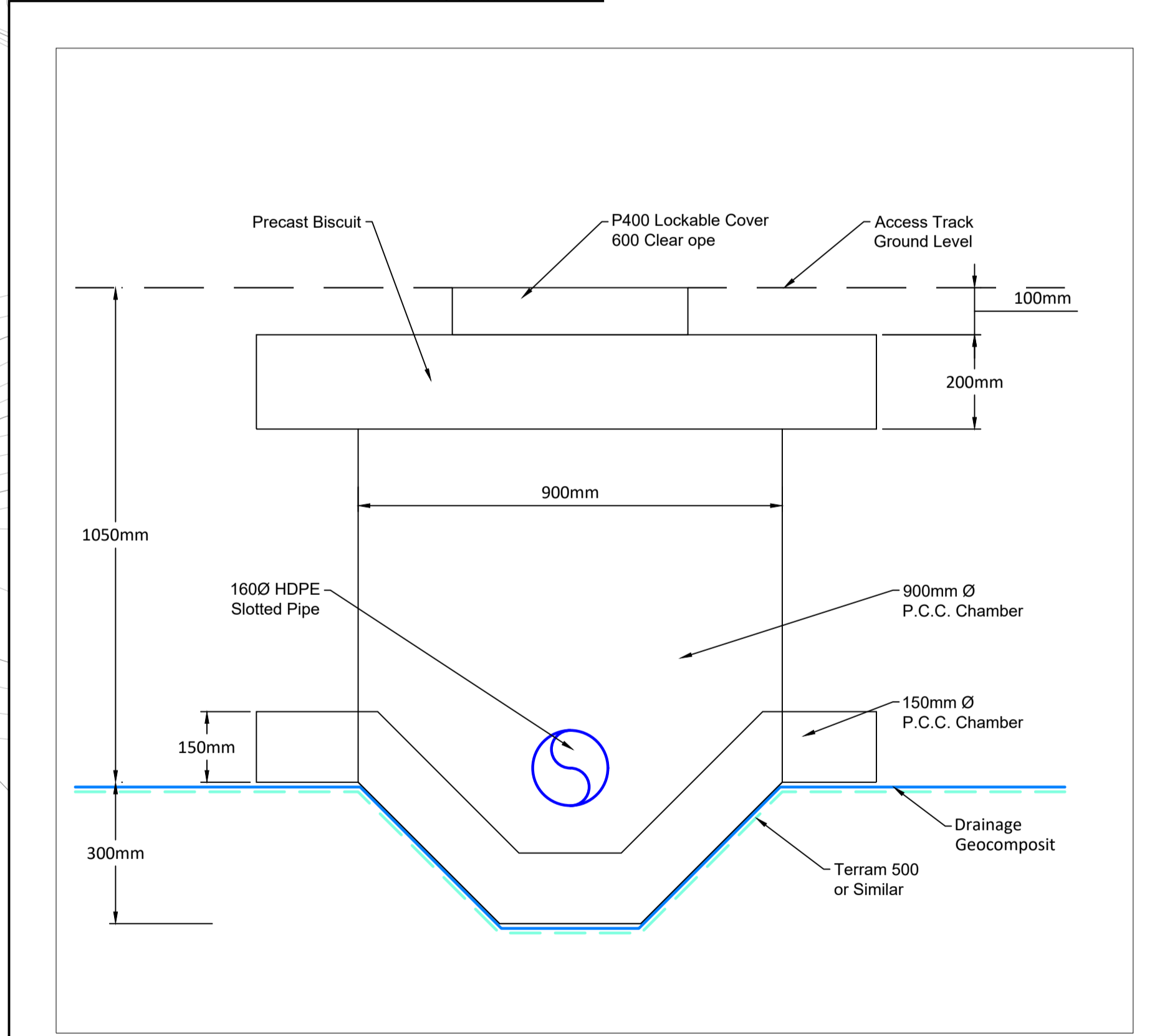
PCC CHAMBER DETAIL Scale 1:10
