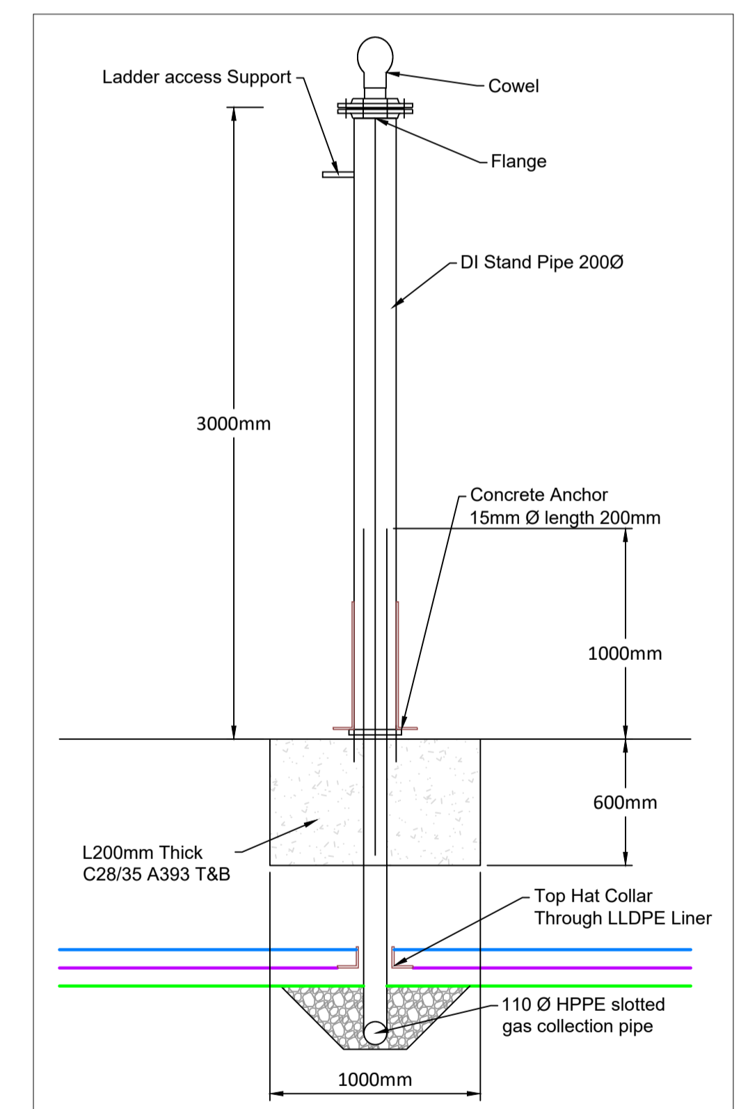
PASSIVE GAS VENT DETAIL
