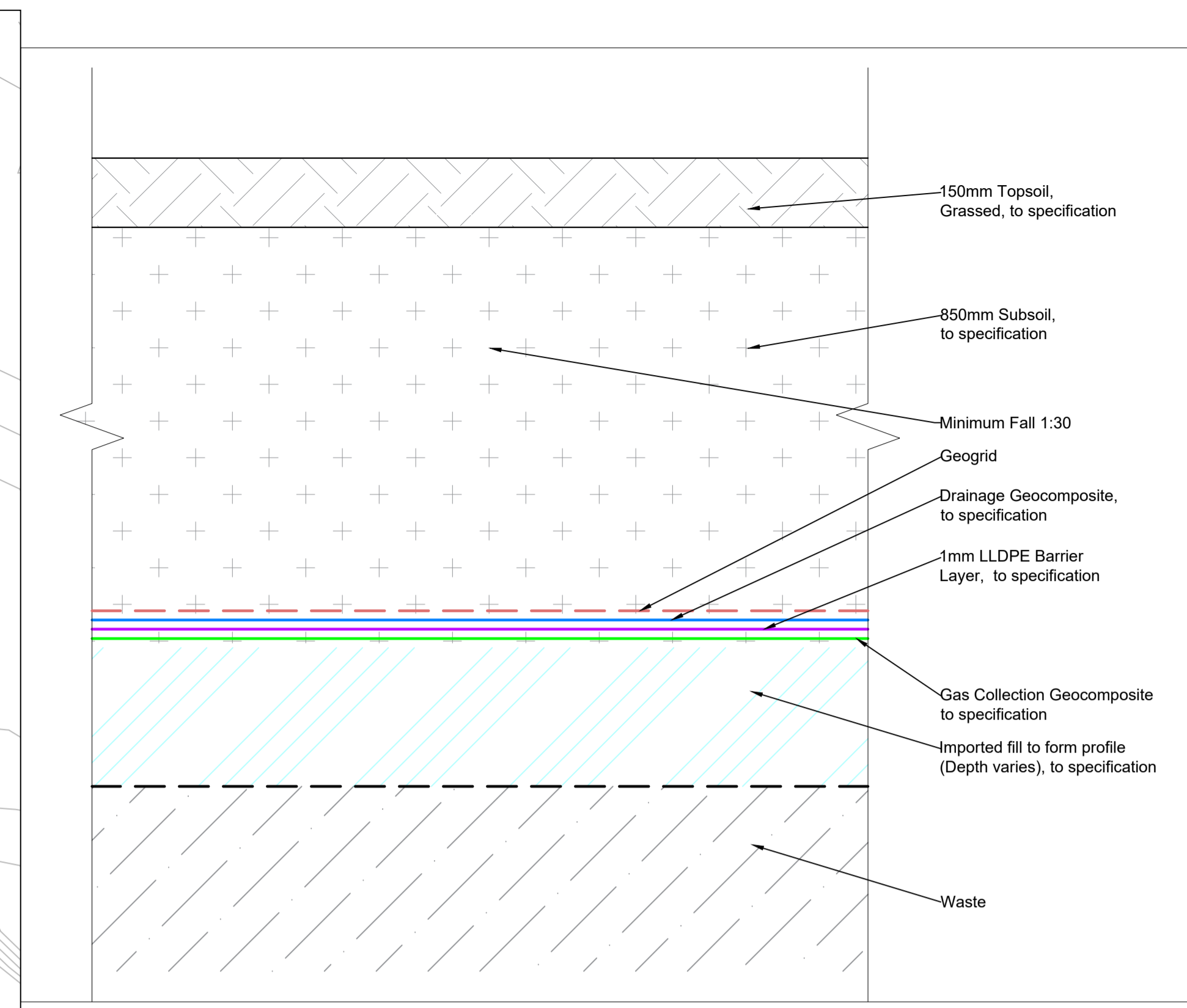
TYPICAL CAPPING DETAIL - WITH GEOGRID
