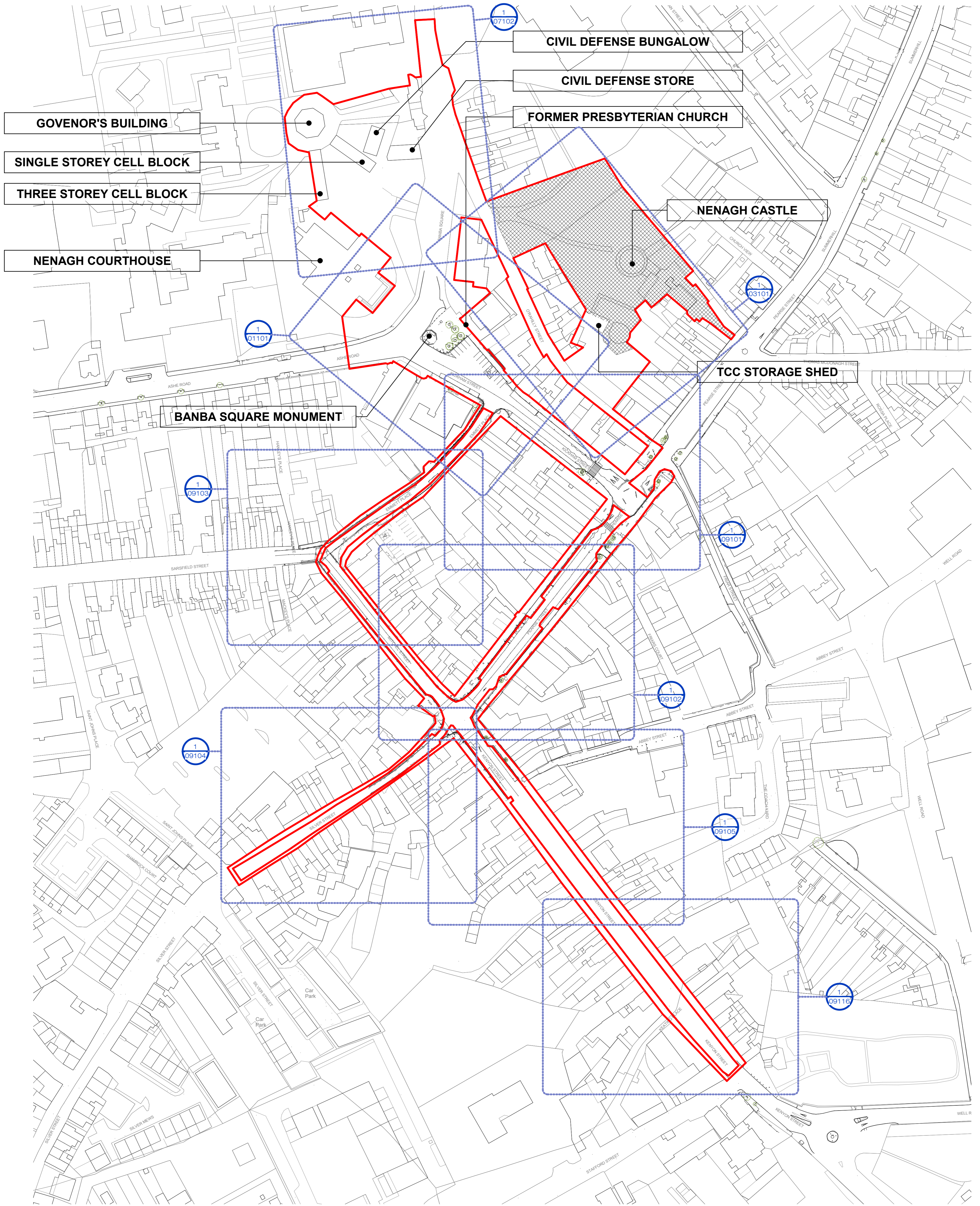
1 EXISTING OVERALL SITE LAYOUT KEY PLAN SCALE: 1 : 1000
