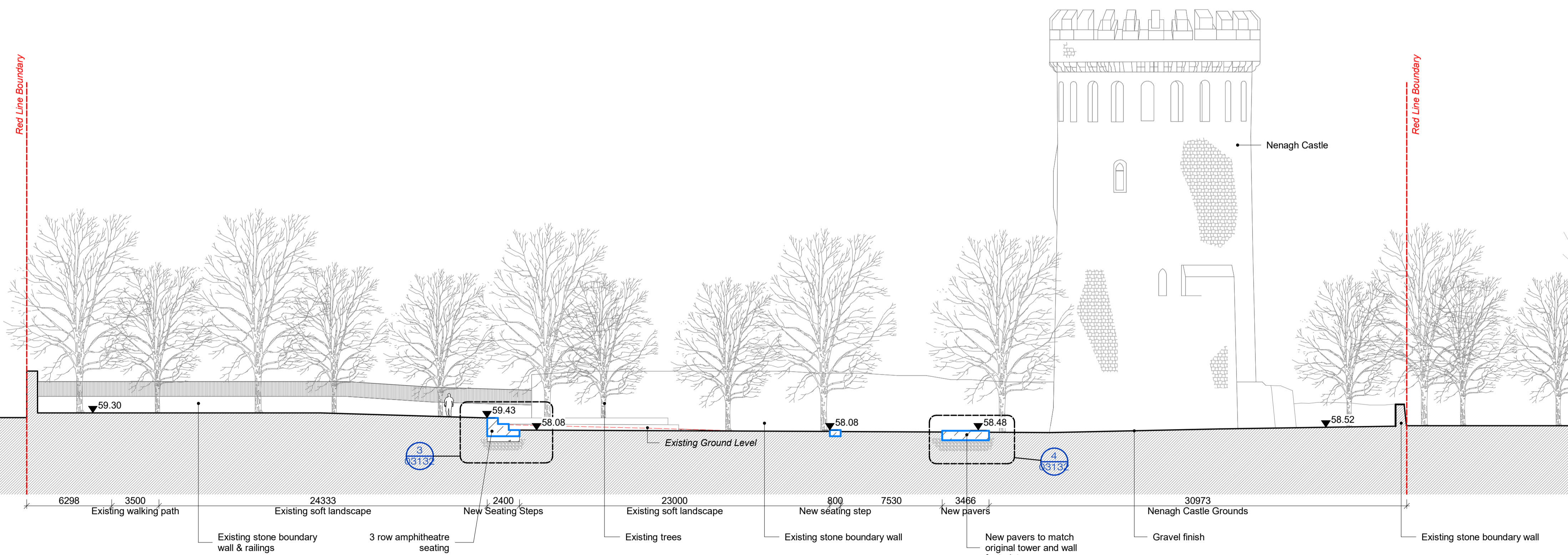
1 CASTLE FIELDS - PROPOSED SITE SECTION SCALE: 1 : 200
