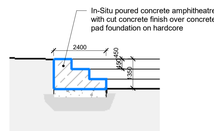
3 SEATING STEP DETAIL SCALE: 1 : 100
