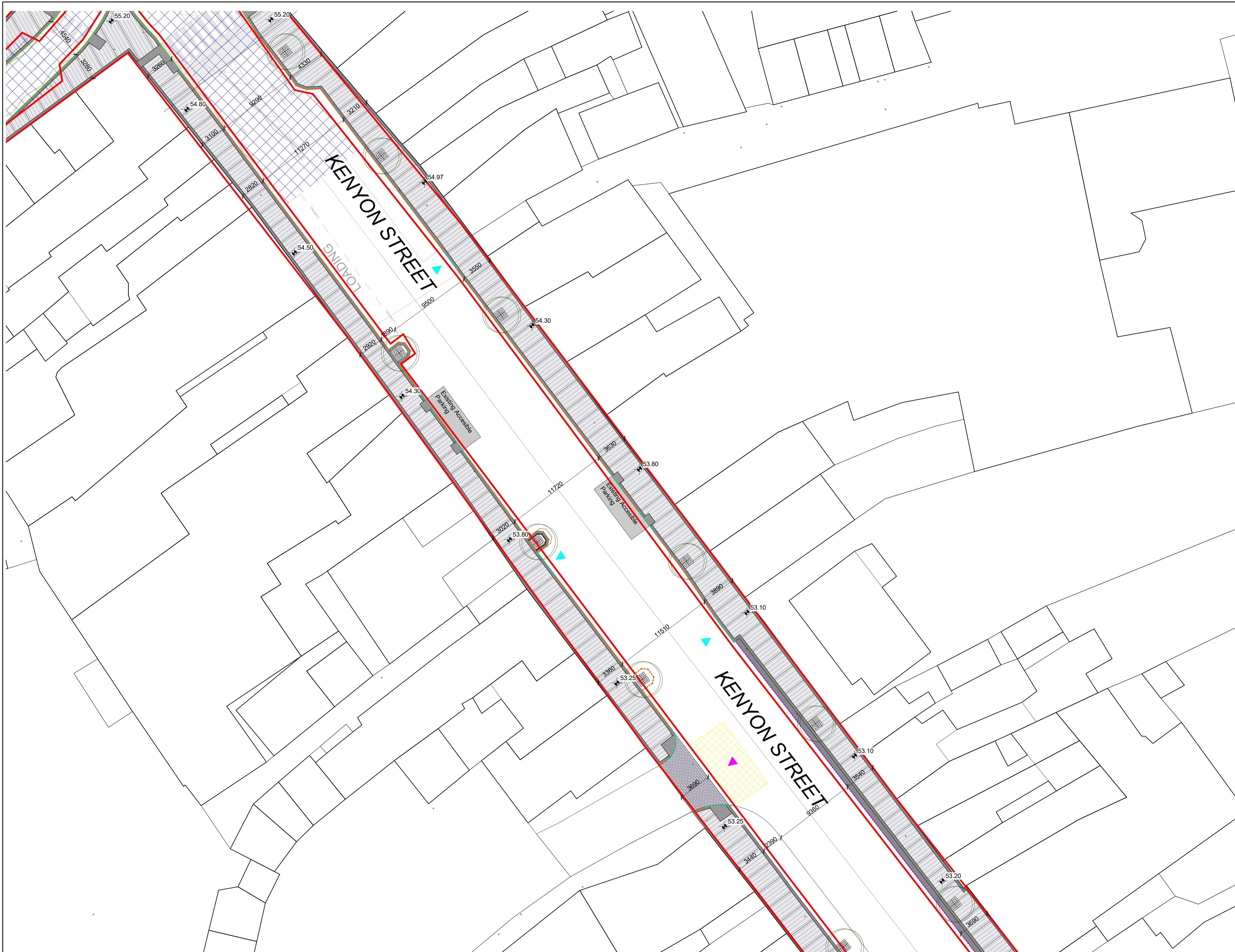
1 PROPOSED ZONE 09 - KENYON STREET NORTH SCALE: 1 : 200
